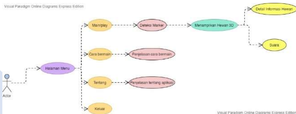
Gambar 21. Use Case Diagram
